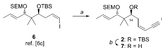
Scheme 4. C9–C19 fragment. Reaction conditions: a ) 1. (trimethylsilyl)acetylene, PdCl 2 (PPh 3 ) 2 , CuI, Et 3 N, CH 3 CN, room temp., 99%; 2. TBAF (1.1 equiv.), THF, 0 °C to room temp., 81%; b ) TBAF (10.0 equiv.), THF, room temp., 95%.
