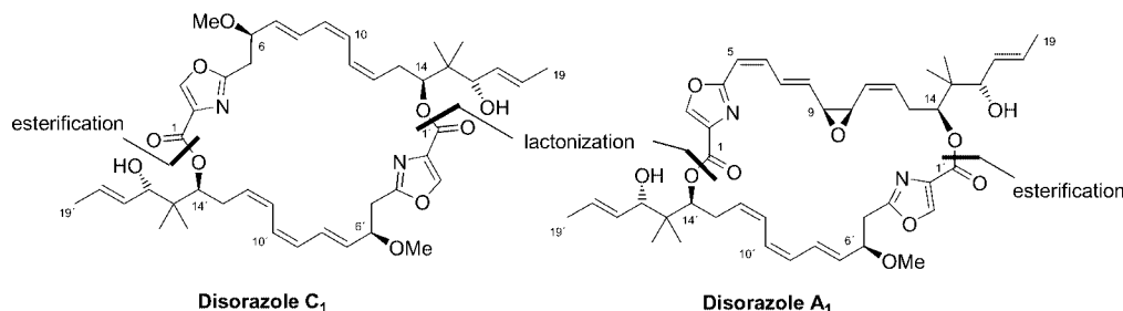
Scheme 1. Cyclization strategy of disorazoles C 1 and A 1 .
