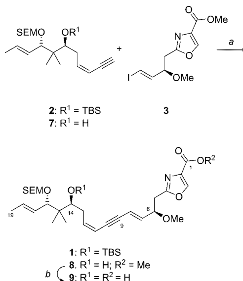
Scheme 5. Fully resolved southern segment. Reaction conditions: a) \text{PdCl}_2(\text{PPh}_3)_2 , CuI, \text{Et}_3\text{N} , DMF, room temp., 77% 1 , 89% 8 ; b) 1.1 N LiOH, THF, room temp., quant.
