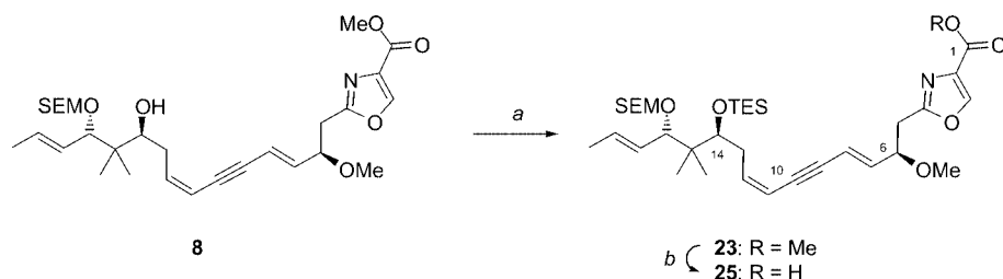
Scheme 10. Protecting group manipulation. Reaction conditions: a) TESOTf, 2,6-lutidine, DMAP, CH 2 Cl 2 , –40 °C to –20 °C, 85%; b) 1 N LiOH, THF, room temp., quant.
