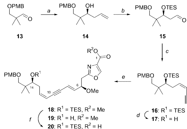
Scheme 7. Simplified C9–C16 fragment. Reaction conditions: a) (+)-Ipc 2 BOMe, allylmagnesium bromide, Et 2 O, –98 °C, 79%, 89% ee; b) 1. TESOTf, 2,6-lutidine, DCM, 0 °C to room temp., 84%; 2. O 3 , PPh 3 , CH 2 Cl 2 , –78 °C to room temp., 85%; c) 1. IPh 3 PCH 2 I, NaHMDS, HMPA, THF, –78 °C to room temp., 72%, Z/E >10:1; 2. CH≡CMgBr, Pd(PPh 3 ) 4 , THF, room temp., 95%; d) TBAF, THF, 0 °C to room temp., 79%; e) PdCl 2 (PPh 3 ) 2 , CuI, 3 , Et 3 N, DMF, room temp., 67% 18 , 81% 19 ; f) 1 N LiOH, THF, room temp., quant. Ipc = Isopinocampheyl.
