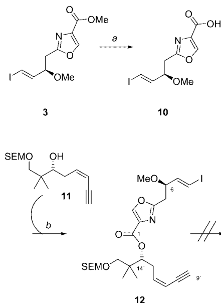
Scheme 6. Alternative cyclodimerization attempt. Reaction conditions: a) LiOH, THF, H 2 O, room temp., quant.; b) 2-chloro-1-methylpyridinium iodide, Et 3 N, DMAP, toluene, 80 °C, 58%.
