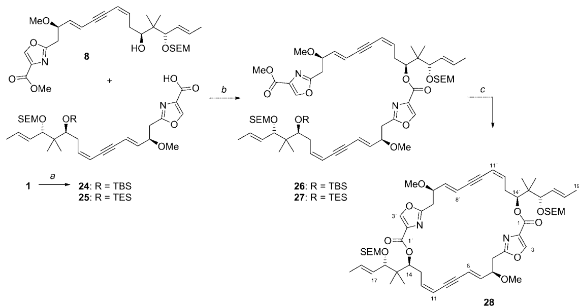
Scheme 9. Synthesis of a disorazole C 1 analogue. Reaction conditions: a) 1 N LiOH, THF, room temp., quant.; b) For 24 : DPTC, DMAP, toluene, reflux, 45%; for 25 : 25 , Cl 3 C 6 H 2 COCl, Et 3 N, toluene, room temp.; 8 , DMAP, toluene, 40 °C, 69%; c) 1. 27 , TBAF, AcOH, H 2 O, THF, room temp., 87%; no reaction for 26 ; 2. Ba(OH) 2 , H 2 O, MeOH, THF, room temp., quant.; 3. Cl 3 C 6 H 2 COCl, Et 3 N, DMAP, toluene, 40 °C, 31%.
