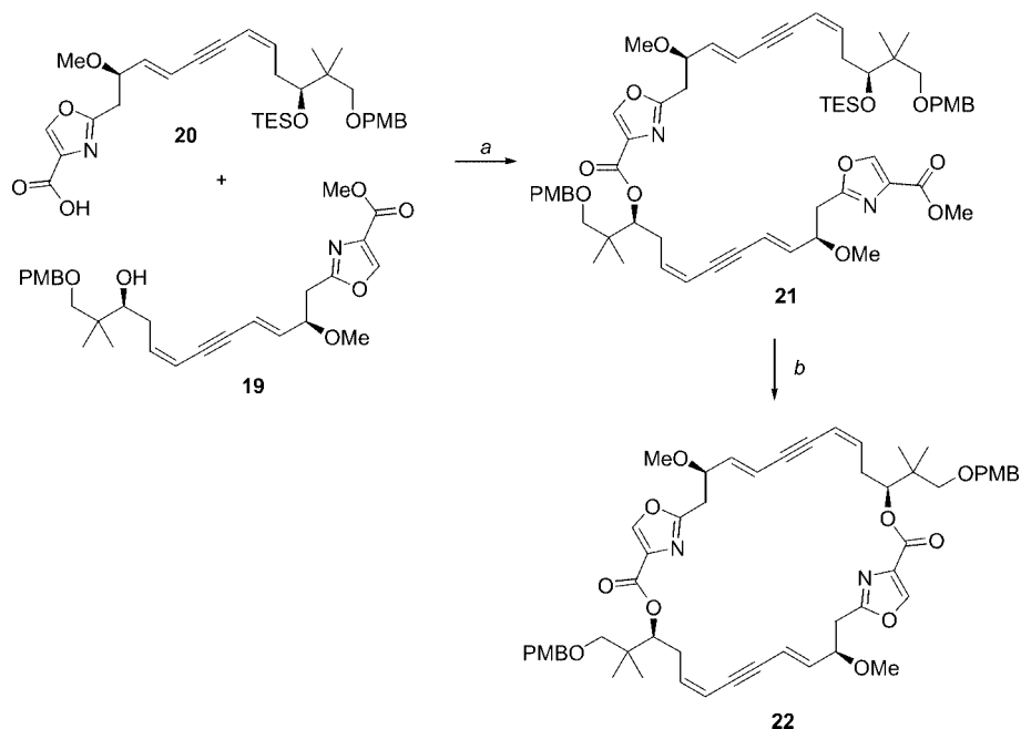
Scheme 8. Cyclisation to the simplified analogue. Reaction conditions: a) Cl 3 C 6 H 2 COCl, Et 3 N, DMAP, toluene, room temp., 8 h, 34%; b) 1. TBAF, AcOH/H 2 O (1:1), THF, room temp., 86%; 2. Ba(OH) 2 , H 2 O, MeOH, THF, room temp., quant.; 3. Cl 3 C 6 H 2 COCl, Et 3 N, DMAP, toluene, room temp., 35%.
