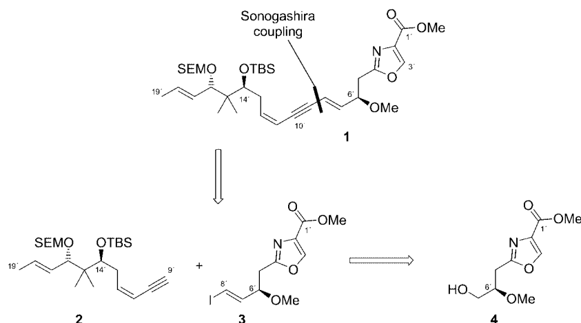
Scheme 2. Retrosynthesis of the southern segment of disorazoles C 1 and A 1 .
