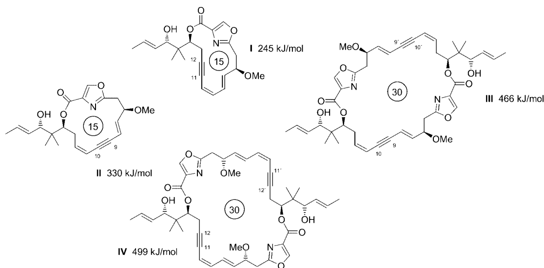
Figure 1. Minimized energies of 15-membered lactones I and II and 30-membered macrodiolides III and IV .
