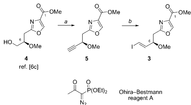
Scheme 3. C1–C8 precursor. Reaction conditions: a ) (ClCO) 2 , Et 3 N, DMSO/CH 2 Cl 2 , –78 °C to –40 °C; then: A , K 2 CO 3 , MeOH, 0 °C to room temp., 75% starting from 4 ; b ) n Bu 3 SnH, Pd(PPh 3 ) 4 , THF, then I 2 , 88%, E -selective.
